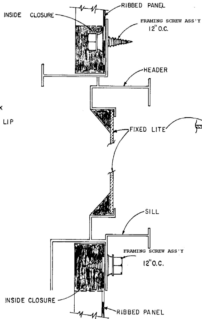
SECTION THRU SILL AND HEADER
