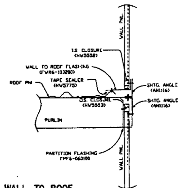
WALL TO ROOF CONNECTION DETAIL (SECTION THRU RAKE, SHEETED BELOW)
