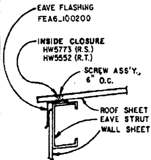
SECTION THRU EAVE (WITH SIDEWALL SHEET)
