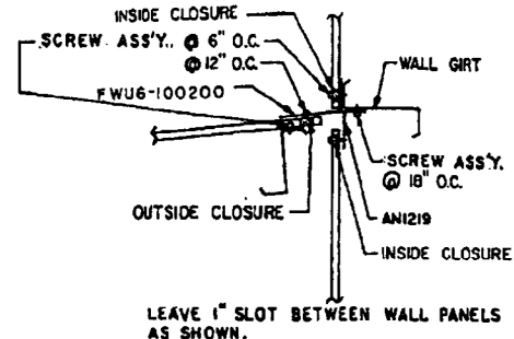
WING UNIT OR CANOPY WALL TO ROOF FLASHING (BELOW EAVE CONDITION)
