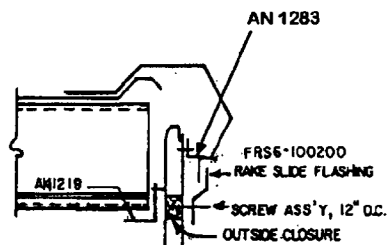
SECTION THRU RAKE WITH RAKE SLIDES
